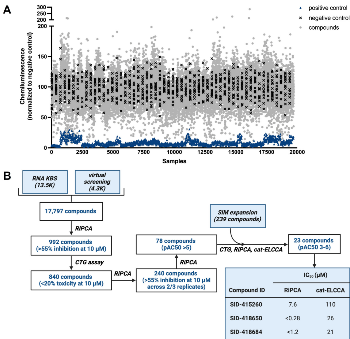
Fig. 2 RiPCA HTS. (A) Campaign view of screening data. (B) HTS funnel and tabulated IC_{50} values for the 3 most active hits in RiPCA and cat-ELCCA.
