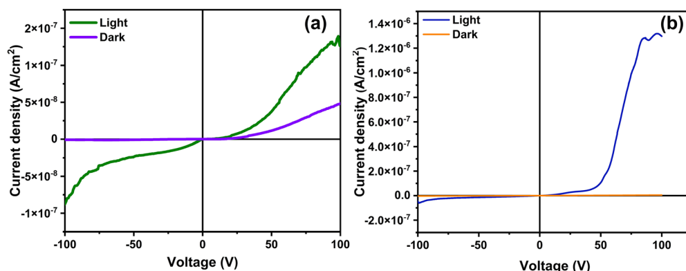
Fig. 5 ( I - V ) photocurrent studies of (a) the undoped \text{CsPbBr}_3 and (b) Bi-doped \text{CsPbBr}_3 perovskite single crystal.
