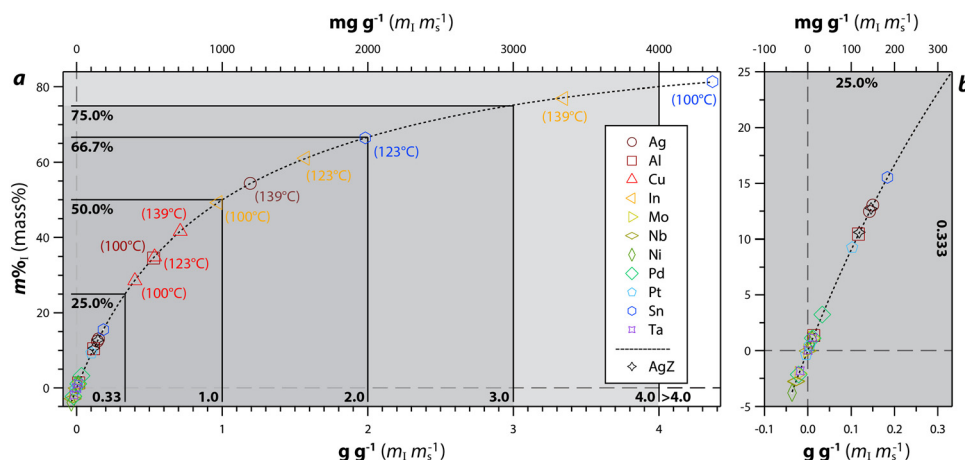
Fig. 9 Data for 100 °C, 123 °C, and 139 °C experiments showing measured iodine ( i.e. , m\% or mass% via EDS) vs. g\ g^{-1} and mg\ g^{-1} along with a double exponential fit including (a) the full plot and (b) the magnified region of \leq 25\ m\% and \leq 0.33\ g\ g^{-1} ( \leq 333\ mg\ g^{-1} ). The highest performing samples are labeled, and the legend is the same for both plots. Reprinted with permission from Riley et al. 122 Copyright 2021 American Chemical Society.
