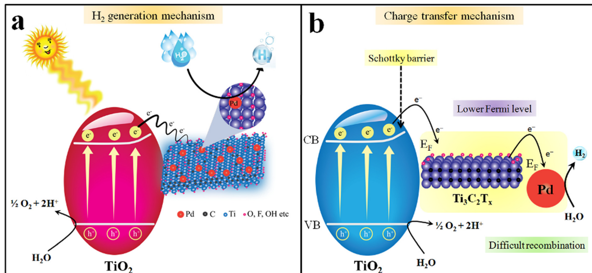
Fig. 10 Mechanism of (a) \text{H}_2 generation. (b) Charge transfer via \text{Pd}@Ti_3C_2T_x-TiO_2 .
