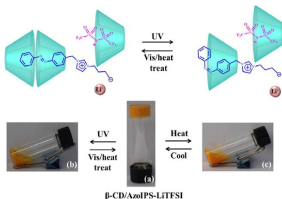
Fig. 47 (a) Mode of inclusion between \beta -CD and AzoIPS-LiTFSI before and after UV irradiation. (b) Preparation of the supramolecular hydrogel: (a) \beta -CD/AzoIPS-LiTFSI (3:1), and its disassembly induced by: (b) UV light, and (c) temperature. Reproduced from ref. 226 with permission from Wiley-VCH, Copyright [2018].
