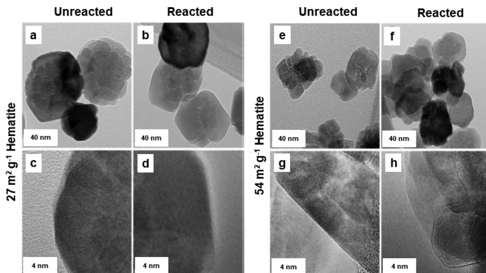
Fig. 48 HRTEM images at two length scales for 27 m² g⁻¹ (a–d) and 54 m² g⁻¹ (e–h) hematite. Reproduced with permission from ref. 292 Copyright 2015, American Chemical Society.
