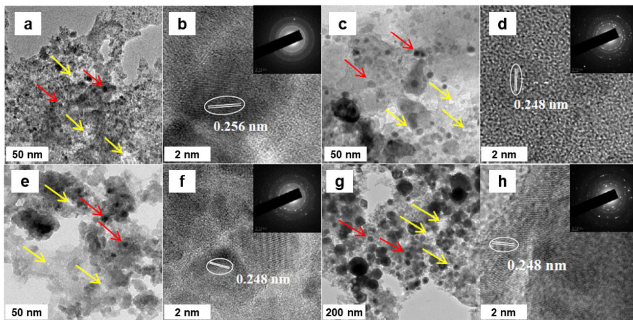
Fig. 67 TEM images of (a, b) \text{Fe}_3\text{O}_4@\text{C}_{350} , (c, d) \text{Fe}_3\text{O}_4@\text{C}_{550} , (e, f) \text{Fe}_3\text{O}_4@\text{C}_{700} , and (g, h) \text{Fe}_3\text{O}_4@\text{C}_{900} nanocomposites (insets: corresponding SAED patterns). Reproduced with permission from ref. 424 Copyright 2013, The Royal Society of Chemistry.
