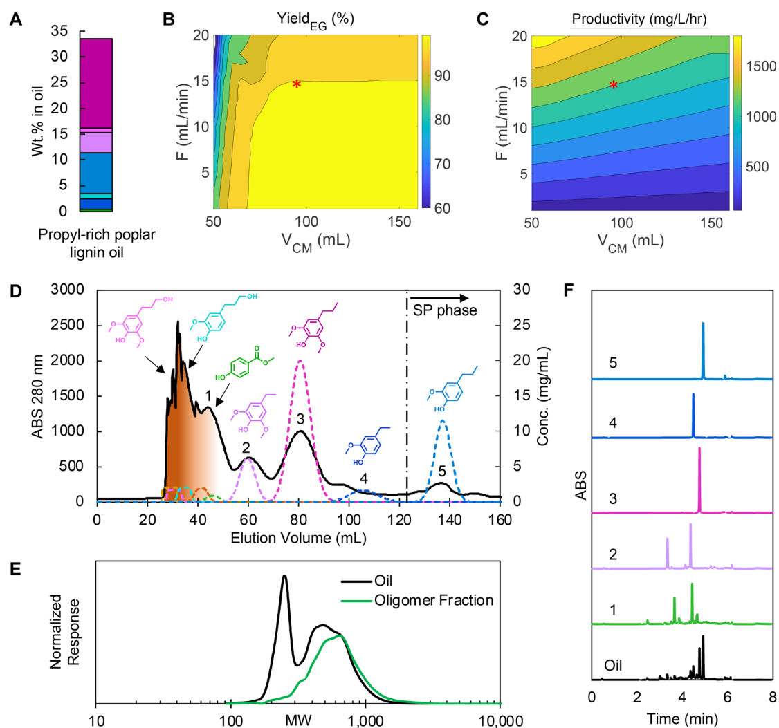
Fig. 8 (A) Monomer composition in propyl-rich poplar lignin oil (colors for each compound match that in Fig. 2), (B) yield prediction of iso Eugenol by varying V_{CM} and flowrate, (C) productivity prediction of iso Eugenol and neighboring pairs by varying V_{CM} and flowrate, (D) CCC chromatogram of the optimized condition, (E) GPC data showing comparison of lignin oil (black) to oligomeric fractions (green), and (F) UHPLC trace analysis of labeled peak fractions in the CCC trace. RCF reaction conditions: 10 g of feedstock, 1 g of Pt/C (5 wt%), 150 mL of methanol/water (50 : 50 v/v), 225 °C, 1 bar of N 2 (at room temperature), and 3 hours after a 30 minutes temperature ramp. CCC operating condition: HEMWat –3 solvent system, head-to-tail flow direction, rotor speed 1400 rpm, feed concentration 200 mg lignin oil per mL, injection volume 6 mL, flowrate 15 mL min -1 and V_{CM} to EECC 95 mL. The feed composition and simulation parameters are listed in Tables S2 and S4,† respectively.
