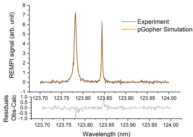
Fig. 2 Experimental (in black) and simulated (in orange) (2 + 1) REMPI spectra of the \text{C}^1\text{B}_1 , v' = 0 \leftarrow \text{X}^1\text{A}_1 , v = 0 transition of HDO in the supersonic beam. See Yang et al. 21 for more details.
