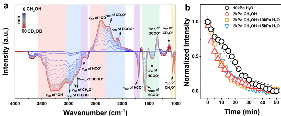
Fig. 4 SSITKA combined with in situ FTIR measurements on NiCe/CN DAC. (a) IR spectra of NiCe/CN DAC recorded at 623\text{ K} during a SSITKA experiment from the initial flow made of 2\text{ kPa CH}_3\text{OH} in Ar to a similar labeled ( 2\text{ kPa CD}_3\text{OD} ) gas-mixture (total flow rate: 50\text{ mL min}^{-1} ). (b) The normalized intensities of surface species in \text{CH}_3\text{OH-CD}_3\text{OD} , \text{H}_2\text{O-D}_2\text{O} and \text{CH}_3\text{OH} + \text{H}_2\text{O-CD}_3\text{OD} + \text{H}_2\text{O} with various pressures of \text{H}_2\text{O} exchange experiments on NiCe/CN DAC as a function of time (black \circ : desorption of \text{DO}^- ; red \triangle : desorption of \text{CH}_3\text{O}^- ; yellow \square : desorption of \text{CH}_3\text{O}^- with 10\text{ kPa H}_2\text{O} co-feed; blue \nabla : desorption of \text{CH}_3\text{O}^- with 15\text{ kPa H}_2\text{O} co-feed). Dotted lines are fitted curves.
