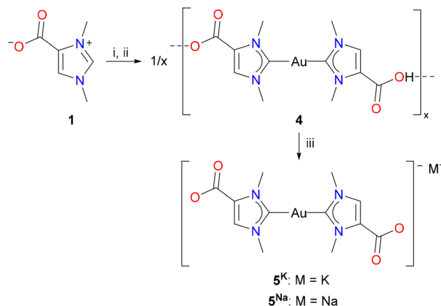
Scheme 3 Preparation of dicarbene gold(I) complexes from norzoanemonin ( 1 ); reagents and reaction conditions: (i) 1 equiv. \text{K}_2\text{CO}_3 , 0.5 equiv. (\text{Me}_2\text{S})\text{AuCl} , MeOH, 12 h, rt; (ii) HI (2 N), pH = 6–7, \text{H}_2\text{O} , rt; (iii) 1 equiv. KOH or NaOH, \text{H}_2\text{O} , rt.
