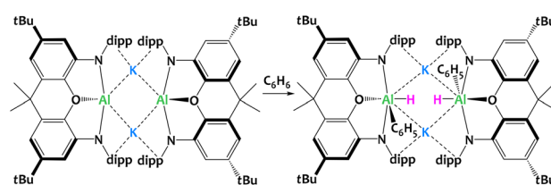
Fig. 31 Formal oxidative addition of the C–H bond in benzene at the \text{Al}^{\text{I}} centres in dimethylxanthene-stabilized potassium aluminyl complex. Dipp = diisopropylphenyl. 119,120
