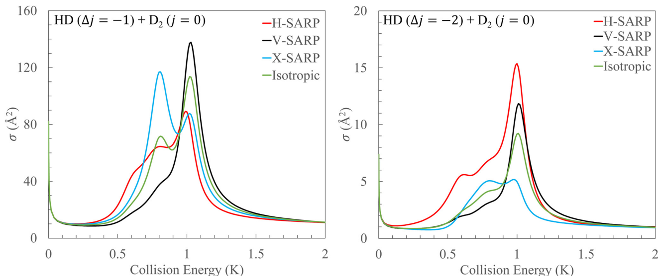
Fig. 10 Integral cross sections as a function of the collision energy for the \nu_{\text{HD}} = 1, j_{\text{HD}} = 2 \rightarrow \nu'_{\text{HD}} = 1, j'_{\text{HD}} = 1 ( \Delta j_{\text{HD}} = -1 ) (left panel) and \nu_{\text{HD}} = 1, j_{\text{HD}} = 2 \rightarrow \nu'_{\text{HD}} = 1, j'_{\text{HD}} = 0 ( \Delta j_{\text{HD}} = -2 ) transitions (right panel) in collision with \text{D}_2(j_{\text{D}_2} = 0) . Green, red, blue, and black colors represent the isotropic, H-SARP, X-SARP, and V-SARP cross sections, respectively.
