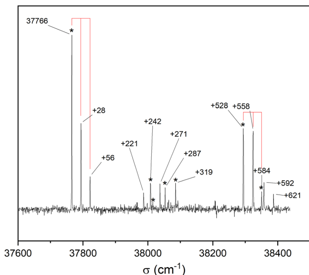
Fig. 3 REMPI S 1 ← S 0 electronic spectrum of the cis -PCD monomer obtained by monitoring its mass at m/z 192 as a function of the laser wavenumber. The 28 cm -1 progression is materialised by vertical lines. The IR-UV spectra were recorded by setting the probe on the electronic transitions indicated by *.
