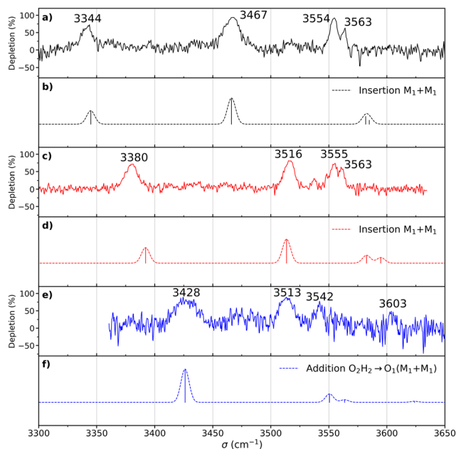
Fig. 6 (a) Experimental double resonance spectrum of the homochiral dimer recorded by setting the probe on the transition origin at 37441 cm -1 . (b) Simulated spectrum of the most stable structure of the homochiral dimer (insertion M 1 + M 1 ). (c) Experimental spectrum of the heterochiral dimer recorded by setting the probe on the transition origin at 37511 cm -1 . (d) Simulated spectrum of the most stable structure (in terms of \Delta E_0 ) of the heterochiral dimer (insertion M 1 + M 1 ). (e) Experimental spectrum of the heterochiral complex recorded by setting the probe on the transition at 37768 cm -1 . (f) Simulated spectra of the most stable structure (judging by \Delta G at 300 K) of the heterochiral dimer (addition O 2 H 2 ··· O 1 (M 1 + M 1 )). The theoretical spectra have been simulated using the scaled harmonic frequencies (scaling factor of 0.963) calculated at the B3LYP-D3(BJ,abc)/ma-def2-TZVP level and convoluted by a Gaussian profile (4 cm -1 FWHM).
