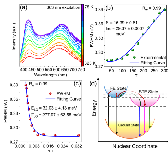
Fig. 3 (a) PL spectra of (5P1)InBr_5 \cdot 2H_2O at various temperatures. (b) and (c) Plots of FWHM (in eV) versus (b) temperature ( T ) and (c) 1/T , along with curves fitted to the data. (d) Schematic diagram for the emission mechanism in (5P1)InBr_5 \cdot 2H_2O . (FE = free exciton, STE = self-trapped exciton).
