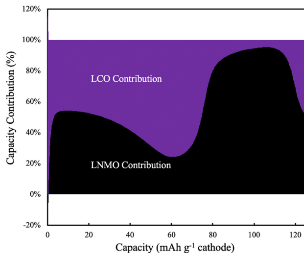
Fig. 6 Simulated capacity contribution from LCO (purple) and LNMO (black) at C/20 discharge (1.13 mA cm -2 ) for the 45%LCO cathode AAM electrode cell.
