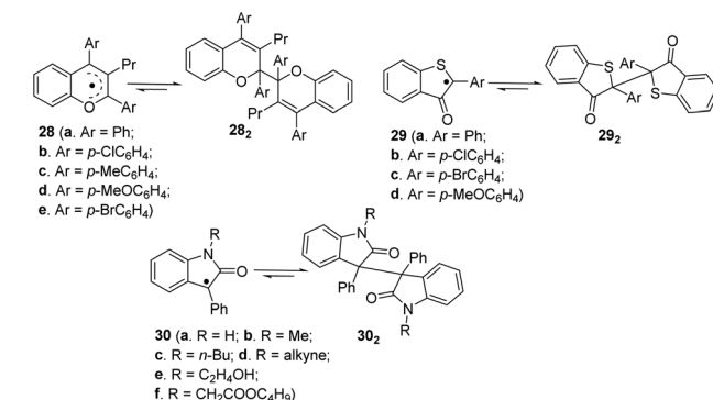
Fig. 11 Carbon-centered radicals with heteroatoms in reversible equilibrium with the dimers (all the conditions for dimers to their corresponding monomers are external force).
