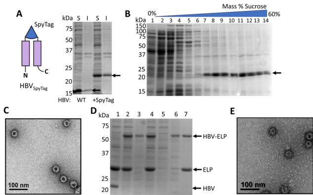
Fig. 2 Incorporation of SpyTag into HBV capsid. (A) SDS-PAGE analysis of soluble (S) and insoluble (I) cell lysates, where full length proteins are denoted with an arrow (B) SDS-PAGE analysis after sucrose gradient analysis of soluble cell lysates; HBV SpyTag is denoted by an arrow. (C) TEM image of HBV SpyTag , pooled from fractions 7–10. (D) SDS-PAGE analysis of HBV SpyTag and ELP 40 -SpyCatcher ligation. (1) HBV SpyTag lysate and purified ELP 40 -SpyCatcher were mixed at a 1:2 molar ratio ( t = 0 ). (2) Post-reaction protein sample. (3) Insoluble proteins after reaction. (4) Soluble proteins after reaction. (5) Soluble contaminants after ITC. (6) Insoluble contaminants after ITC. (7) Purified conjugates after one cycle of ITC. (E) TEM image of purified conjugates after one cycle of ITC.
