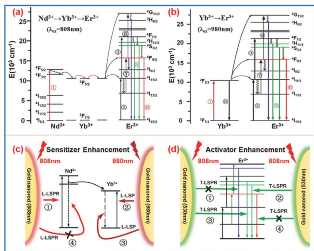
Fig. 3 (a and b) The energy diagrams of Nd 3+ , Yb 3+ , and Er 3+ ions undergoing ETU upon excitation at 808 and 980 nm, respectively. (c) The GNR Longitudinal-SPR-induced absorption enhancement for an Nd 3+ ion upon excitation at 808 nm and for a Yb 3+ ion upon excitation at 980 nm. The radiative decay rate of the Yb 3+ ion is also accelerated by the GNR Longitudinal-SPR (due to energy matching) while that of the Nd 3+ ion is not (denoted by “x”) because of the fast phonon-mediated relaxation and energy migration to the Yb 3+ ion. (d) The GNR Transverse-SPR-induced green-emission enhancement for both ions upon excitation at 808 nm. The blue and red emissions are not affected by the GNR Transverse-SPR due to energy mismatch (denoted by “x”). 75
