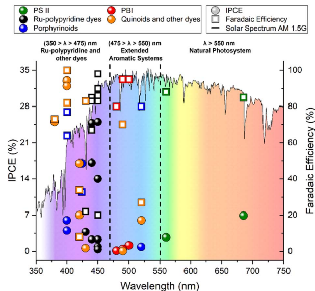
Fig. 28 Plot of IPCE (circles; only the maximum values are reported) and FE (empty squares) as the key performance parameters representing the photon-to-current and current-to-oxygen performance, respectively. From this plot, it is evident that: (i) best performing systems exploit high energy radiation ( \lambda < 475 nm), as in the case of Ru-polypyridine chromophores; (ii) porphyrinoids and organic dyes overstepping this barrier ( \lambda between 475 and 550 nm) are still associated with low IPCE values; (iii) the “green region” above 550 nm where the PSII operates is almost unexploited in artificial systems.
