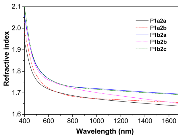
Fig. 3 Wavelength-dependent refractive indices of the thin films of P1a2a – P1b2c .
