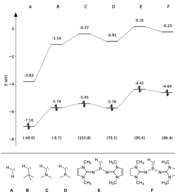
Fig. 4 Eigenenergies of the HOMO and LUMO for carbenes A – F obtained at the B3LYP-GD3BJ/def2-TZVP level. The respective singlet–triplet energy differences ( \Delta E_{\text{ST}} ) are given in parentheses.
