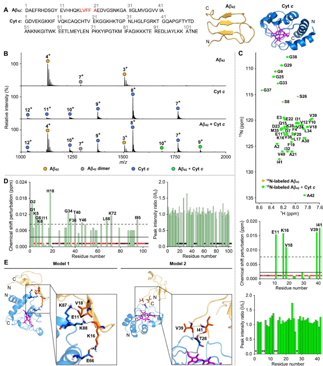
Fig. 2 Interaction between Cyt c and Aβ 42 . (A) Amino acid sequences and structures of Cyt c (PDB 1HRC) 28 and Aβ 42 . 29 The heme group in Cyt c and the self-recognition site of Aβ 42 are highlighted in pink and red, respectively. (B) Complexation between Cyt c and Aβ 42 detected by ESI-MS. Conditions: [Aβ 42 ] = 100 μM; [Cyt c ] = 100 μM; 20 mM ammonium acetate, pH 7.4; 37 °C; incubation for 30 min. The samples were diluted by 10-fold prior to injection to the mass spectrometer. (C) Two-dimensional (2D) 1 H- 15 N band-selective optimized flip angle short transient-heteronuclear multiple quantum correlation (SOFAS-HMQC) NMR spectra (800 MHz) of 15 N-labeled Aβ 42 monomer with and without Cyt c . The average of chemical shift perturbations (CSPs) and the average plus one standard deviation are presented with solid and dashed lines, respectively. Black asterisks represent the amino acid residues that cannot be resolved for analysis, and red asterisks indicate the amino acid residues without detectable CSPs. Conditions: [ 15 N-labeled Aβ 42 ] = 40 μM; [Cyt c ] = 200 μM; 150 mM HEPES, pH 7.4; 10% v/v D 2 O; 10 °C. (D) Analysis of the CSPs and the change in the peak intensity observed within 15 N-labeled Cyt c by addition of Aβ 42 . The 2D 1 H- 15 N heteronuclear single quantum coherence (HSQC) NMR spectra of 15 N-labeled Cyt c with and without Aβ 42 monomer are depicted in Fig. S7.† (E) Representative models of the Cyt c -Aβ 42 interfaces from the trajectories of MD simulations. Initial conformations of Cyt c (PDB 1HRC; blue) 28 and Aβ 42 (yellow) 29 were used for binding studies. The heme group in Cyt c is highlighted in pink. Model 1 and 2 of the Cyt c -Aβ 42 adducts are illustrated in Fig. S9.† Possible hydrogen bonds are depicted with dashed black lines.
