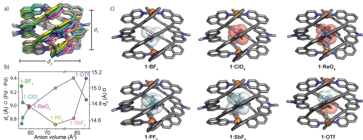
Fig. 3 Solid-state comparison of 1 \cdot X : (a) an overlay of the six X-ray structures of 1 (the structures are centred on Pd1, and counter-ions and hexyl chains are removed for clarity). d_1 = \text{Pd} \cdots \text{Pd} separation, d_2 = average distance between carbazole-N atoms.; (b) a plot of the solid-state structural parameters obtained from single-crystal X-ray analysis. Anion volumes were calculated by DFT geometry optimizations (RB3LYP; B, O, F, Cl, P, S: 6-31g(d); Re, Sb: LANL2DZ); (c) X-ray crystal structures of 1 \cdot X . Hexyl chains, hydrogen atoms and unbound anions are omitted for clarity.
