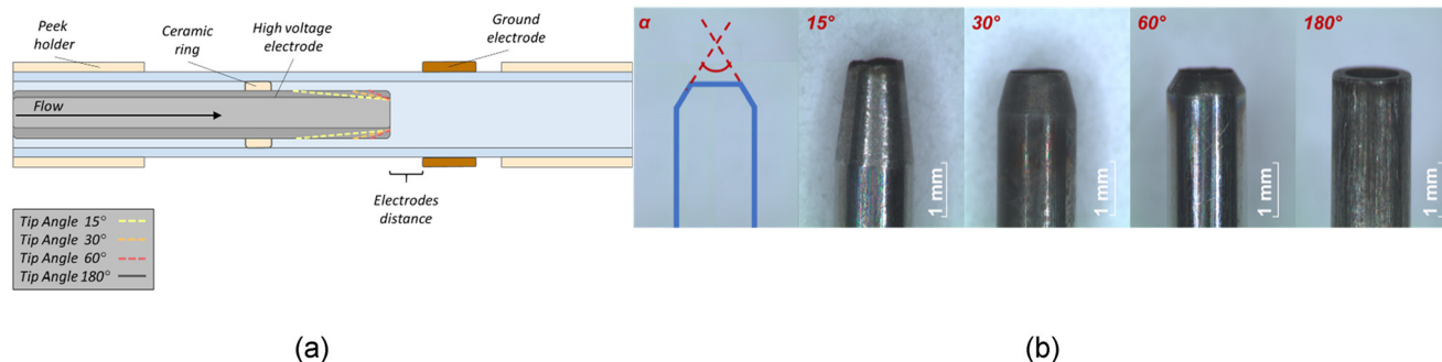
Fig. 1 (a) Schematic drawing of plasma jet reactor with key design parameters indicated, including the images at the stereomicroscope of the high voltage electrodes manufactured with different tip angles (b).
