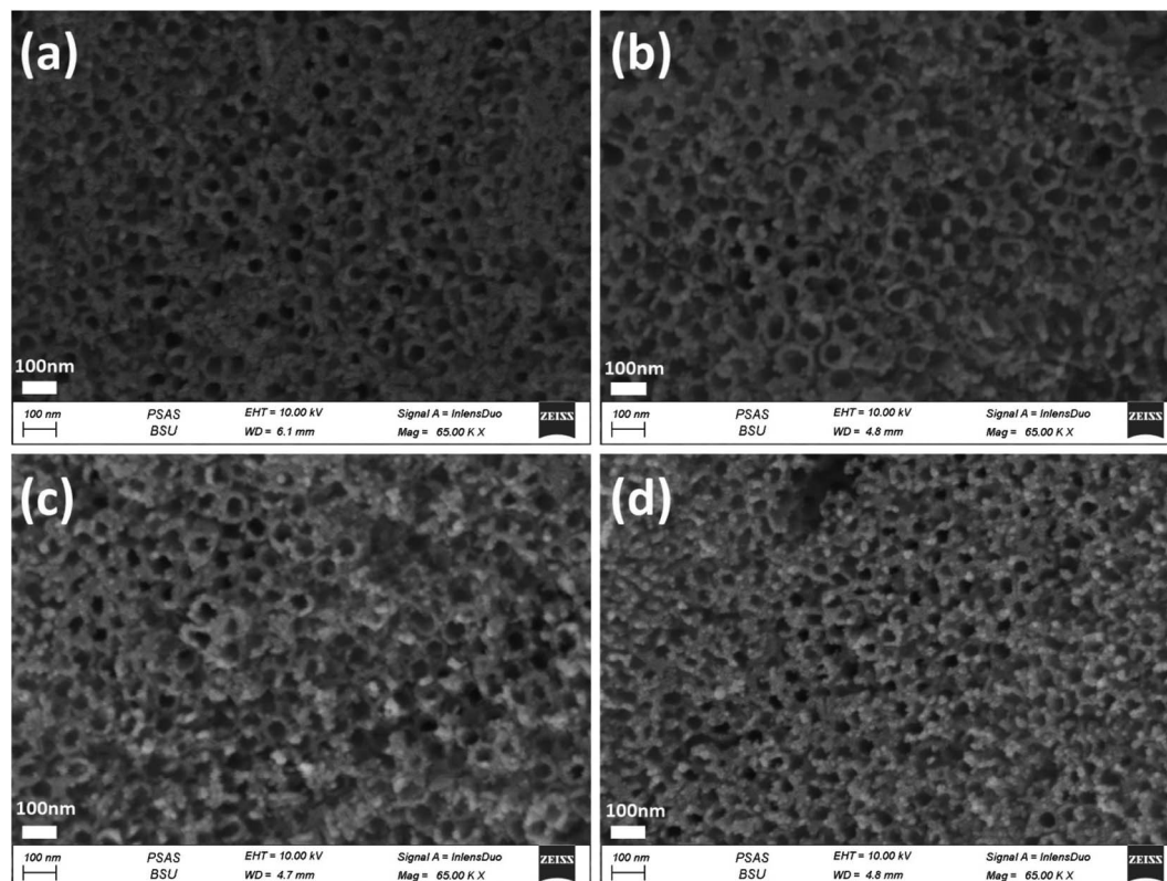
Fig. 4 FESEM images of the top-view of \text{Au}_y/\text{Ni}_{20}/\text{TiO}_2\text{NTs} photoanodes synthesised by different time intervals of photodeposition (a) 15 min, (b) 30 min, (c) 60 min and (d) 120 min.
