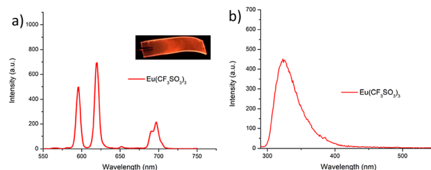
Fig. 9 (a) The \text{Eu}(\text{III}) -centred emission observed for F2 when measured in \text{H}_2\text{O} . (b) The corresponding fluorescence spectrum of F2 measured in \text{H}_2\text{O} . Inset (a) photograph of polymer following soaking for 10 min in \text{Eu}(\text{CF}_3\text{SO}_3)_3 solution under UV-irradiation showing the characteristic red luminescence from \text{Eu}(\text{III}) .
