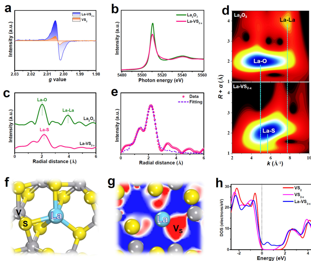
Fig. 2 (a) EPR spectra of \text{VS}_2 and \text{La-VS}_{2-x} . (b) \text{La L}_3 -edge XANES, (c) EXAFS spectra and (d) WT profiles of \text{La-VS}_{2-x} and reference \text{La}_2\text{O}_3 . (e) EXAFS fitting curve of \text{La-VS}_{2-x} and (f) the corresponding fitting model. (g) Electron contour map of \text{La-VS}_{2-x} (red: charge accumulation, blue: charge depletion). (h) DOS plots of \text{VS}_2 , \text{VS}_{2-x} and \text{La-VS}_{2-x} .
