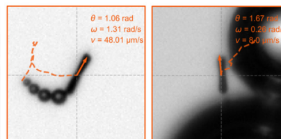
Fig. 3 Deep learning-based micromotor tracking. Simulation and training: (A) Example of a simulated micromotor image generated by DeepTrack 2.1. 33,34 Each image (256 px × 256 px) contains one or more micromotors with aspect ratios similar to those used in the experiments. Bubbles of different sizes (smaller bubbles trailing behind the rods, and larger bubbles in the background) are added to make the images look realistic and thereby closer to the experimental images (see the experimental images in (D) and (G)). For each input image (A), a corresponding output image with a segmentation map (C) is also generated to separate the micromotors from the background and the bubbles. (B) U-Net architecture: A U-Net is employed to transform the input simulated image into the segmentation map. The architectural details and information on each block are indicated in the legend. Inference and analysis: the U-Net model trained on simulated images is then applied on experimental images (D) generating the segmentation maps of the micromotors (E). The positions and orientations of the micromotors are obtained from the segmentation maps. (F) Trajectories: by extracting the positions of all the frames in a video, the trajectories of the micromotors are measured. (G) Each trajectory is further processed to calculate the linear velocities ( v ) and angular velocities ( \omega ). Individual micromotor trajectories are represented in the orange boxes.
