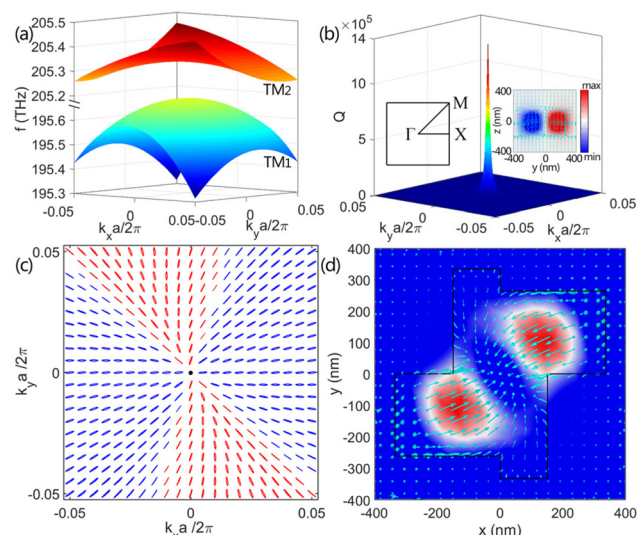
Fig. 2 The eigenmode analysis of the isolated periodic chiral metasurface. (a) The simulated transverse magnetic (TM) band structures. (b) The calculated Q -factors of the TM_1 band. The radiative Q -factor diverges at the \Gamma point, indicating the occurrence of a symmetry-protected BIC. The left inset denotes the schematic of first Brillouin zone of a square lattice. The right inset shows the magnetic field ( H_x ) distributions on the x = 0 nm slice for the symmetry-protected BIC. The arrows indicate the electric field vector. (c) The eigen polarization map at the first Brillouin zone for the TM_1 band. The polarization states are represented by ellipses. The red and blue colors correspond to the left-handed and right-handed states, respectively. The black dot denotes a vortex polarization singularity, known as the unique BIC. (d) The magnetic field distributions at the plane of z = 0 nm for the symmetry-protected BIC. Overlaid on the colour map is the plot of the electric field vector denoted by the light blue arrows.
