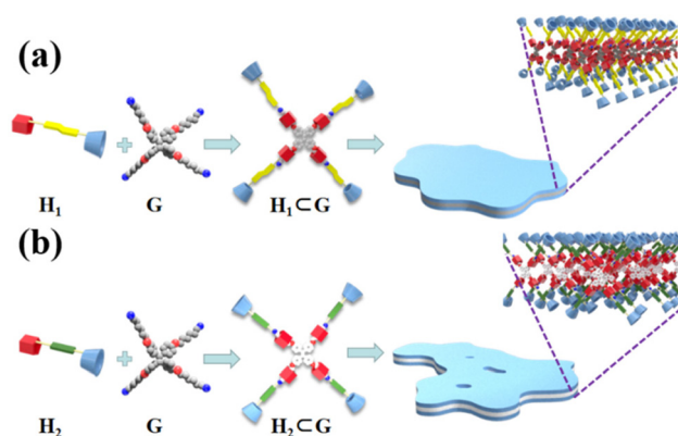
Fig. 10 Formation of host-guest complexes (a) H 1 C 2 G and (b) H 2 C 2 G , and self-assembly in \text{CHCl}_3/\text{DMSO} solution, respectively.
