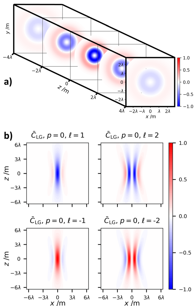
Fig. 9 (a) 3D plot showing the variation of the polarisation independent C_{LG} for a beam with \ell = 2, p = 0 along the propagation axis. (b) 2D plot showing the diffractive properties of the polarisation independent optical chirality density of LG beams, which stemming purely from longitudinal fields means C_{LG} = \bar{C}_{LG}^{\parallel} . In all plots w_0 = \lambda .
