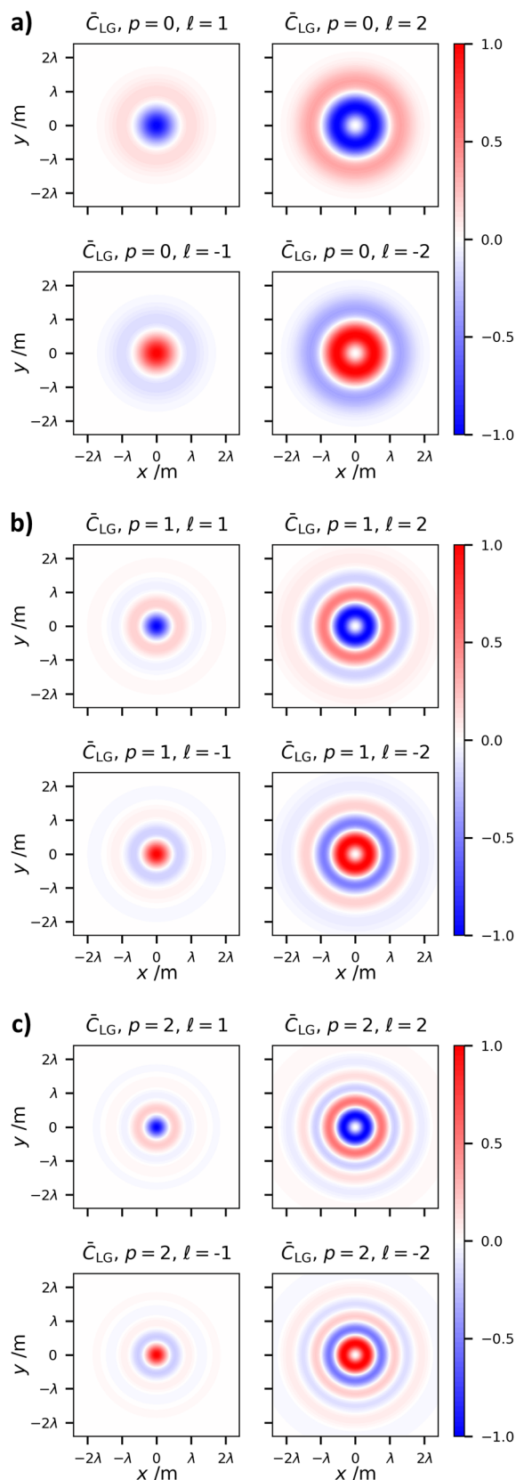
Fig. 8 Optical chirality densities for both linearly polarised and unpolarised LG modes where (a) p = 0 , (b) p = 1 and (c) p = 2 . In all cases the optical chirality densities stem purely from the longitudinal fields, that is \bar{C}_{LG} = \bar{C}_{LG}^{\parallel} and \bar{C}_{LG}^{\perp} = 0 . In all plots w_0 = \lambda .
