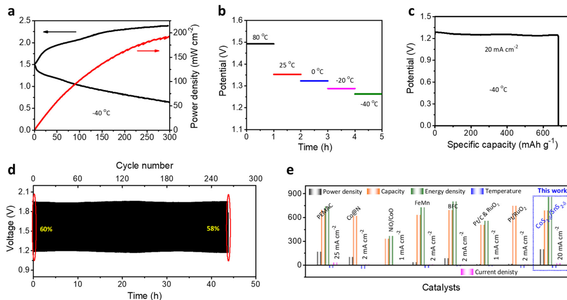
Fig. 8 All temperature performance of flexible ZABs. (a) LSV and power density measurements of \text{CoS}_{1-\delta}/\text{SnS}_{2-\delta} at -40^\circ\text{C} . (b) Discharge rate voltages for wide operating temperatures from 80 to -40^\circ\text{C} at 10\text{ mA cm}^{-2} . (c) Capacity and energy density for \text{CoS}_{1-\delta}/\text{SnS}_{2-\delta} at -40^\circ\text{C} for 20\text{ mA cm}^{-2} . (d) Cycle life performance for \text{CoS}_{1-\delta}/\text{SnS}_{2-\delta} -based Zn-air cells for -40^\circ\text{C} at 50\text{ mA cm}^{-2} . (Time: 10 min per cycle.) (e) Ragone plots projecting the state-of-the-art cell capacities and power/energy densities ( i.e. , capacity ( \text{mAh g}^{-1} ), power ( \text{mW cm}^{-2} ), energy ( \text{Wh kg}^{-1} ), temperature ( ^\circ\text{C} ), and current densities ( \text{mA cm}^{-2} )) related to those of previous reports for sub-zero temperatures.
