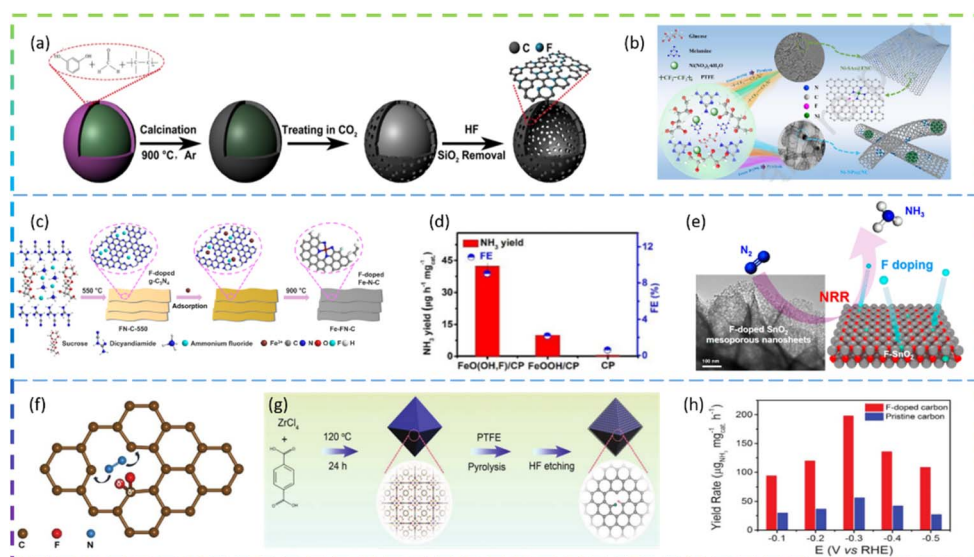
Fig. 5 (a) Schematic illustration to the formation process of the fluorine-doped cage-like porous carbon (F-CPC). (b) Schematic illustration for the formation and structures of Ni-SAs@FNC and Ni-NPs@FNC. (c) Schematic diagram for the synthesis of Fe-FN-C. (d) NH 3 yields and FEs of different electrodes at -0.60 V after electrolysis for 2 h. (e) Schematic diagram of electrocatalytic reduction of N 2 on fluorine-doped SnO 2 porous nanosheets. (f) Schematic of the atomic structure of fluorine-doped carbon. (g) Schematic of the synthetic procedure for F-doped carbon. (h) Yield rate for NH 3 of F-doped carbon and pristine carbon at different applied potentials.
