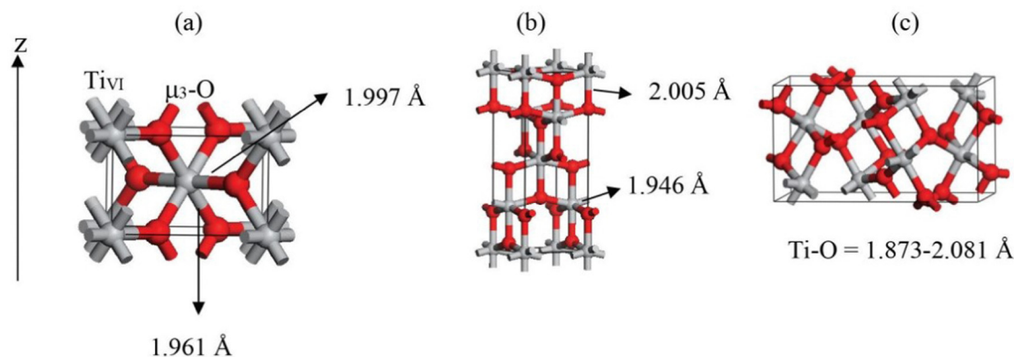
Fig. 2 Structures of TiO 2 natural polymorphs: (a) rutile, (b) anatase and (c) brookite. 17
