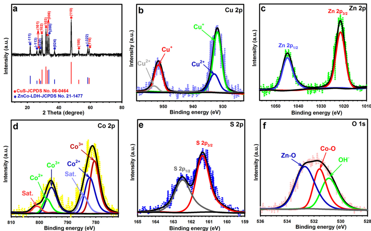
Fig. 4 (a) XRD pattern of CS10-ZC-LDH4. (b) Cu 2p XPS spectra of CS10-ZC-LDH4. (c) Zn 2p XPS spectra of CS10-ZC-LDH4. (d) Co 2p XPS spectra of CS10-ZC-LDH4. (e) S 2p XPS spectra of CS10-ZC-LDH4. (f) O 1s XPS spectra of CS10-ZC-LDH4.
