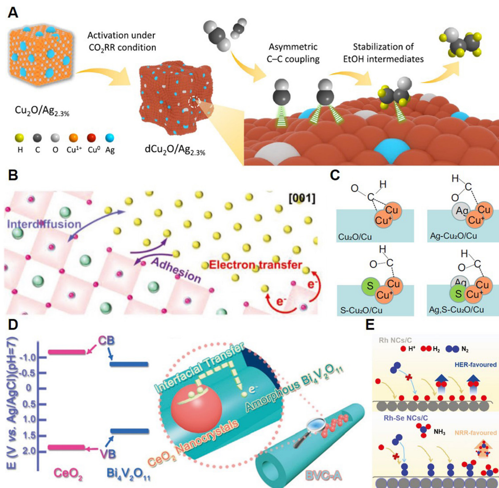
Fig. 3 (A) Illustration of promoted \text{CO}_2 -to- \text{C}_2\text{H}_5\text{OH} on a \text{dCu}_2\text{O}/\text{Ag}_{2.3\%} electrocatalyst. Reprinted with permission from ref. 29. Copyright 2022, Springer Nature; (B) Interaction between perovskite oxides and Cu nanoparticles. Reprinted with permission from ref. 30. Copyright 2022, John Wiley & Sons, Inc.; (C) *CHO intermediates on different Cu-based electrocatalysts. Reprinted with permission from ref. 31. Copyright 2022, Springer Nature; (D) Schematic for interfacial charge transfer in BVC-A. Reprinted with permission from ref. 33. Copyright 2018, John Wiley & Sons, Inc.; (E) Different NRR pathways on Rh-based catalysts before and after adding the Se component. Reprinted with permission from ref. 34. Copyright 2020, John Wiley & Sons, Inc.
