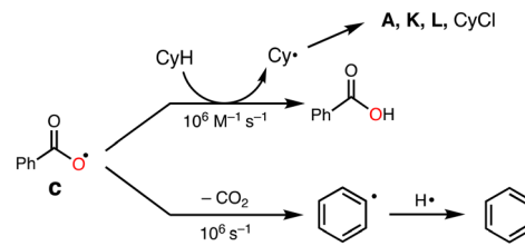
Scheme 4 Competition of HAA with decarboxylation from c .
