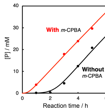
Fig. 4 Time courses of the cyclohexane oxidation by the \text{O}_2 /PhCHO system with and without m -CPBA (10 mM). Reaction conditions: [\text{1}] = 0.025 mM, [\text{PhCHO}] = 0.2 M, [\text{cyclohexane}] = 2.0 M at 40 °C under \text{O}_2 .
