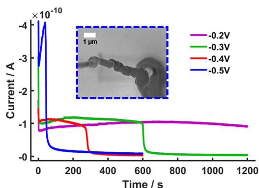
Fig. 3 i vs. t plots recorded during the potentiostatic ( E_{\text{app}} = -0.20 to -0.50 V) single-barrel SECCM eATRP/FRP of Am using [Am]:[HEBiB]:[ \text{Cu}^{\text{II}} ]:[TPMA] = [20]:[1]:[0.5]:[0.625]; (inset) SEM image of a gel-like feature formed when E_{\text{app}} = -0.50 V.
