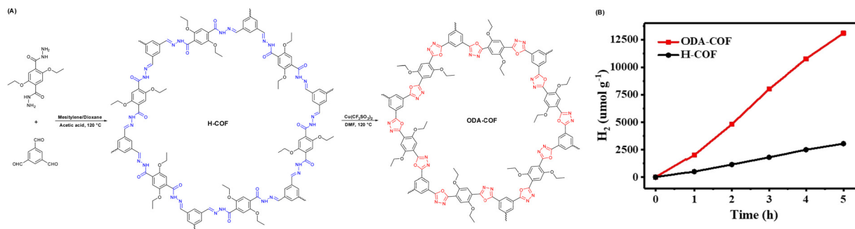
Fig. 11 (A) Synthesis representation and chemical structure of H-COF and ODA-COF. (B) Time course of photocatalytic \text{H}_2 evolution capability for H-COF and ODA-COF. Reprinted with permission, copyright, 2022, Wiley-VCH. 91
