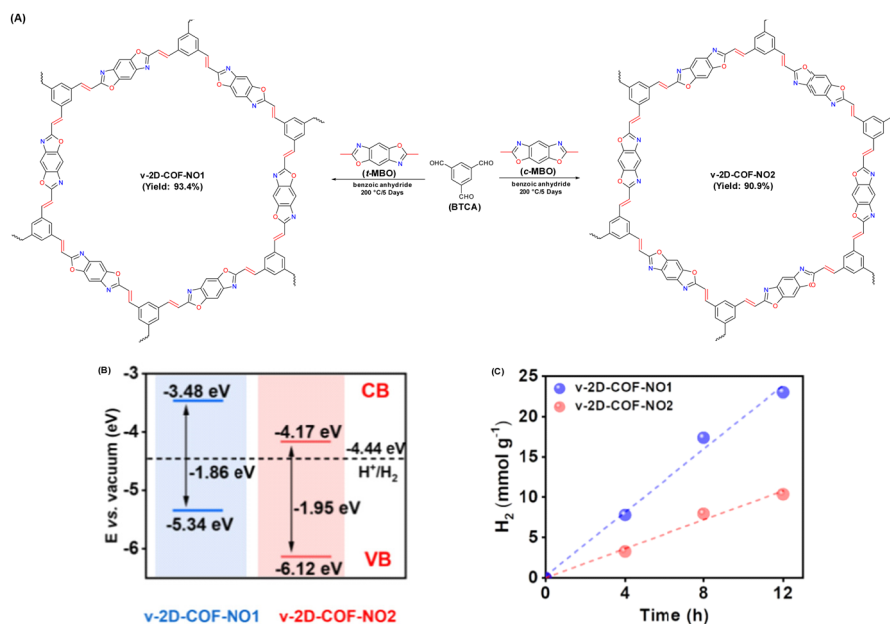
Fig. 12 (A) Schematic illustration for establishing v-2D-COF-NO1 and v-2D-COF-NO2. (B) Energy band position of v-2D-COFNO1 and v-2D-COF-NO2. (C) Time course of photocatalytic \text{H}_2 production activity for v-2D-COFNO1 and v-2D-COF-NO2. Reproduced with permission, copyright, 2022, American Chemical Society. 94
