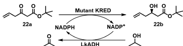
Scheme 9 Biosynthesis of tert -butyl ( R )-3-hydroxy-5-hexenoate 22b .
