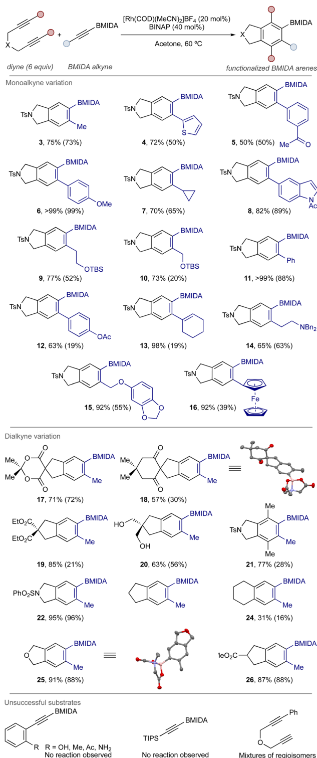
Scheme 2 Example scope of the cycloaddition process. Monoalkyne component indicated in blue in products. Yields determined by ^1\text{H} NMR, isolated yields (chromatography and/or crystallization) in brackets. See ESI† for full details.
