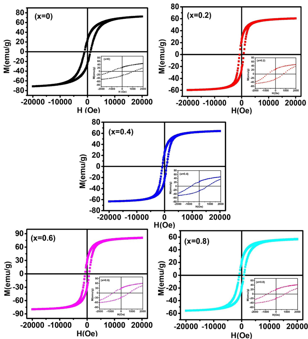
Fig. 15 Room temperature hysteresis ( M - H ) loops of \text{Co}_{1-x}\text{Mn}_x\text{Fe}_2\text{O}_4 ( 0.8 \geq x \geq 0 ) NF samples. The inset of the figure shows an enlarged view closer to the center. The lower values of coercivity indicate the single-domain particles.
