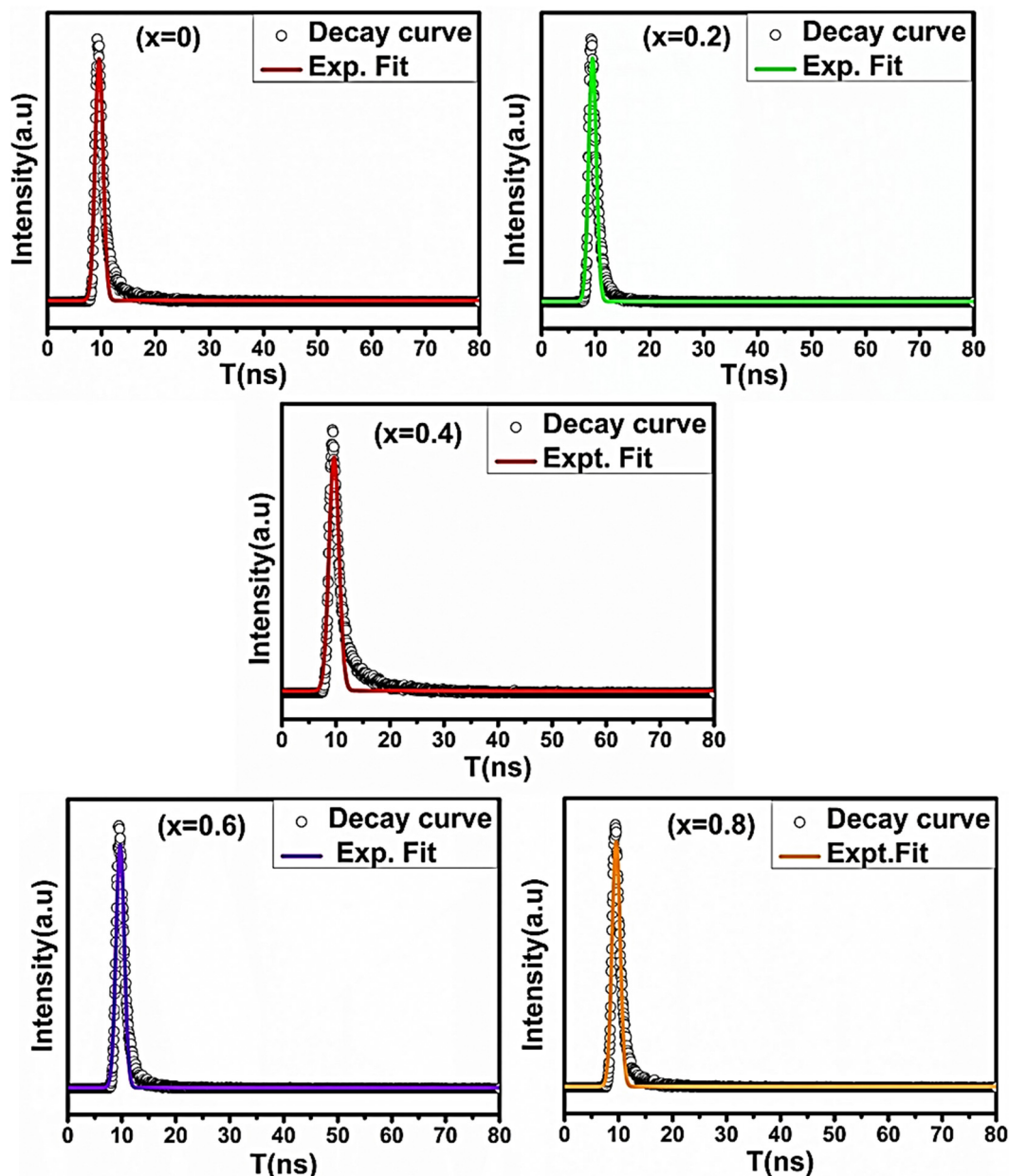
Fig. 14 Room temperature time-resolved photoluminescence spectra (hollow symbols) and double exponentially fitted spectrum (solid lines) of the \text{Co}_{1-x}\text{Mn}_x\text{Fe}_2\text{O}_4 ( 0 \leq x \leq 0.8 ) NF samples.
