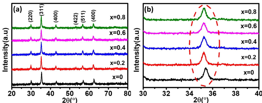
Fig. 2 (a) X-Ray diffraction spectra of \text{Co}_{1-x}\text{Mn}_x\text{Fe}_2\text{O}_4 ( 0.8 \leq x \leq 0 ) nanoferrites. (b) Enlarged view of major diffraction peak of (311) plane XRD spectra of all the samples. All samples show good crystalline behavior and their major peaks shifted towards the lower 2\theta values with an increase in \text{Mn}^{2+} ion concentration.
