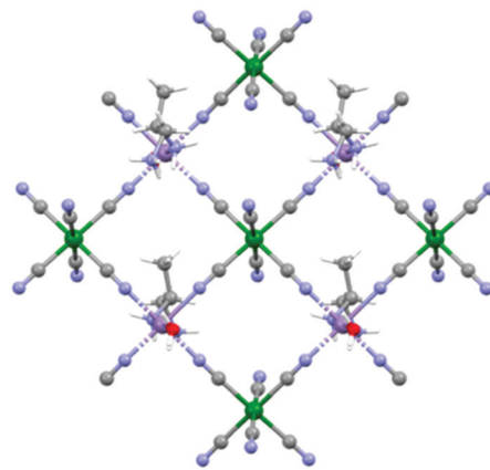
Fig. 3 View of the squared 2D-layers of 1 that develop along the ab crystallographic plane. Color codes: violet, \text{Mn}^{\text{II}} ; green, \text{Cr}^{\text{III}} ; red, O; light-blue, N; gray, C; white, H.
