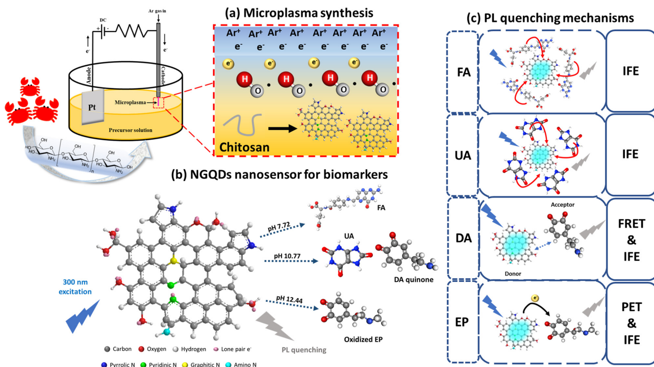
Scheme 1 Microplasma synthesis of bioresource NGQDs for biomarker detection. (a) Microplasma synthesis of NGQDs from chitosan. (b) PL-based selective detection of FA, UA, DA, and EP by adjusting the pH value using NGQDs. (c) PL quenching mechanisms of NGQDs, including an inner filter effect (IFE) for FA at pH 7.72, IFE for UA at pH 10.77, Förster resonance energy transfer (FRET) for DA at pH 10.77, and oxidative photoinduced electron transfer (PET) for EP at pH 12.44. By exploiting the excitation-dependent behavior of NGQDs coupled under the pH conditions, the IFE mechanism can be maximized to yield the selective and sensitive detection of UA, FA, EP, and DA.
