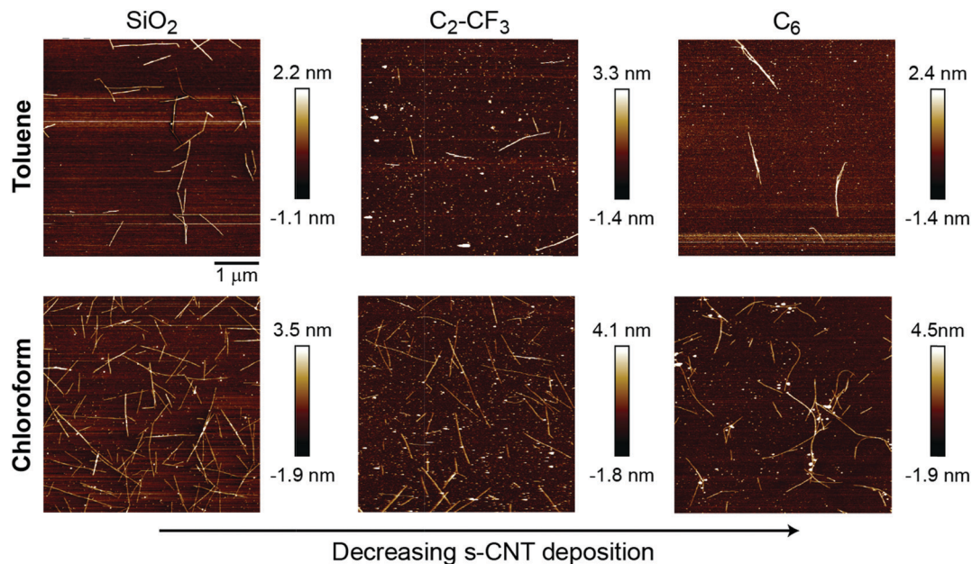
Fig. 4 Representative atomic force microscopy images of PFO-BPy-wrapped s-CNTs deposited on bare SiO 2 or surfaces grafted with C 2 -CF 3 or C 6 SAMs. Deposition was quantified for 2 \mu\text{g mL}^{-1} s-CNTs in either toluene (top row) and chloroform (bottom row) ink. s-CNTs are visible as thin white lines in the AFM images.
