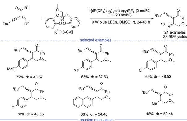
Scheme 6 Cu-catalyzed regioselective 1,4-carboacylation of 1,3-enynes with redox-active esters.
