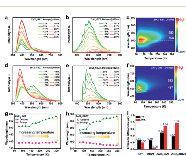
Fig. 3 Temperature-dependent spectra and time-resolved decay measurements. Prompt and delayed spectra of \text{ZnCl}_2\text{-BZT} (a, b and c) and \text{ZnCl}_2\text{-CBZT} (d, e and f) at different temperatures ranging from 77 K to 297 K. Comparison of dominant emission positions of \text{ZnCl}_2\text{-BZT} (g) and \text{ZnCl}_2\text{-CBZT} (h) under prompt and delayed modes. (i) Calculated differences between dominant emission peaks under prompt and delayed modes for BZT, CBZT, \text{ZnCl}_2\text{-BZT} , and \text{ZnCl}_2\text{-CBZT} at 77 K and 297 K.
