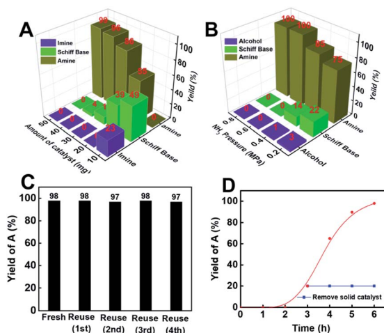
Fig. 3 (A) Effect of the catalyst amount, (B) effect of NH 3 pressure, (C) reusability of Co@C-N(800), and (D) time–yield plots for reductive amination of cyclohexanone with Co@C-N(800) (red line) and removing Co@C-N(800) after 3 h (blue line). Reaction conditions: cyclohexanone, 1 mmol; methanol, 3 mL; 35 °C; 6 h; Co@C-N(800), 50 mg (29.2 mol% Co); total pressure of NH 3 and H 2 was 2 MPa and 1.4 MPa H 2 and 0.6 MPa NH 3 in part D.
