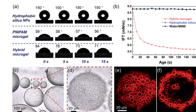
Fig. 2 (a) Contact angles of a water drop on the films of the hydrophobic silica NPs, PNIPAM microgels, and hybrid microgels. (b) Dynamic interfacial tension between water and MtBE without (▲) or with the hybrid microgel (●) and hydrophobic silica NPs (■). (c and d) Optical micrographs of the w/o Pickering emulsion stabilized by the hybrid microgels. (e and f) CLSM images of the hybrid microgels at the w/o interface observed from different focus points.
