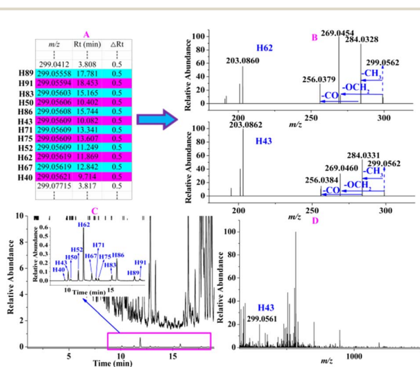
Fig. 6 An example of characterization flavonoids with low intensity. (A) In the constructed precursor ion list, twelve compounds ( H40 , H43 , H50 , H52 , H62 , H67 , H71 , H75 , H83 , H86 , H89 , and H91 ) were extracted at m/z 299.0556–299.0562; (B) performing targeted MS/MS analysis to obtain the fragmentation ions, such as H43 and H62 ; (C) the twelve compounds were covered by other high intensity ingredients and exhibited relative abundances of not more than 0.7% in a full scan; (D) the relative abundances of the precursor ions of these twelve ingredients were lower or much lower than those of others in MS spectra, such as H43 .
